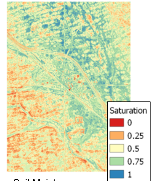
Soil Moisture
