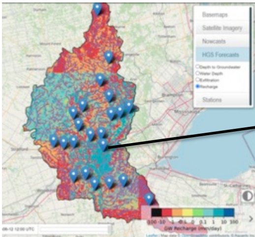
Groundwater Recharge
