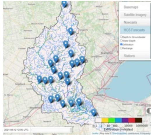
Groundwater Discharge
